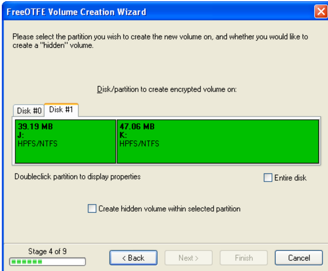
New volume wizard showing full partition information
