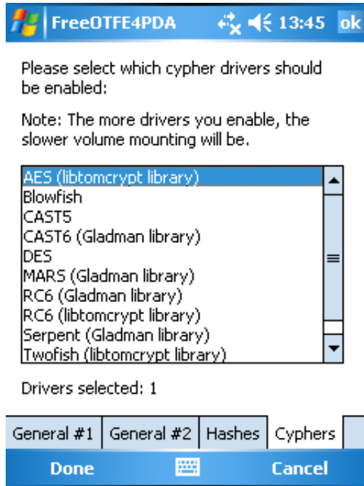
Options dialog; enabling/disabling cypher drivers
