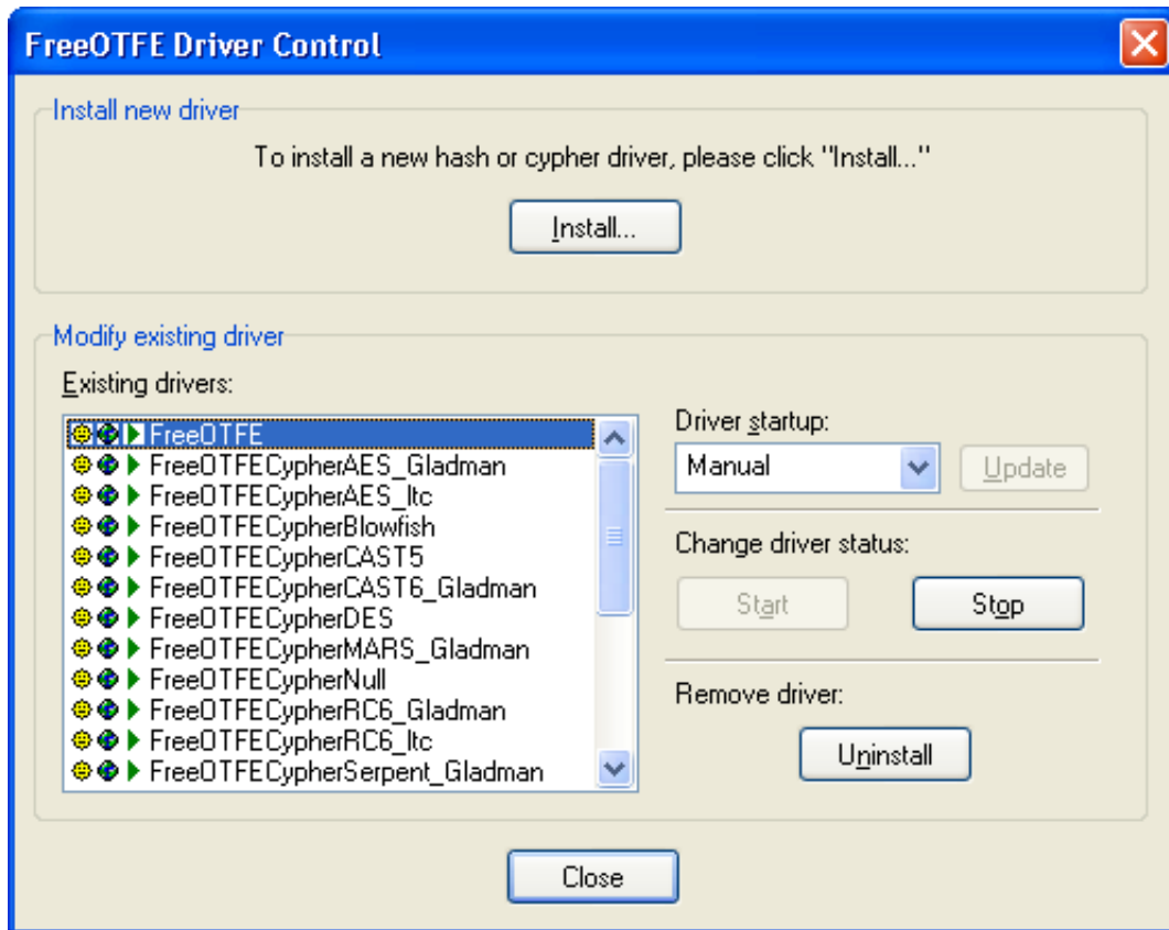
Driver control dialog
